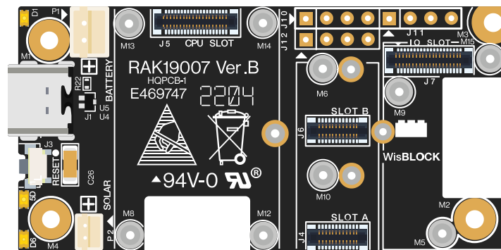
Figure 1: WisBlock Base Board 2nd Gen top view
